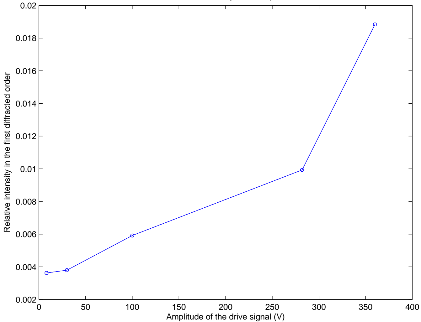
Diffraction efficiency vs. drive power
