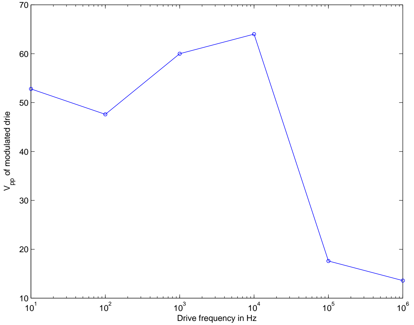
Frequency response of AOM driver
