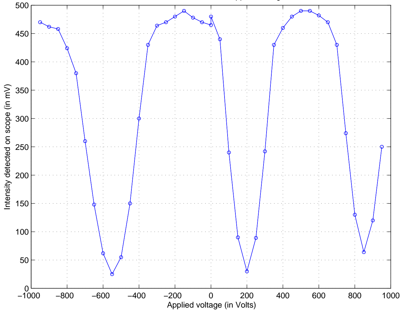
EOM transmission versus applied voltage
