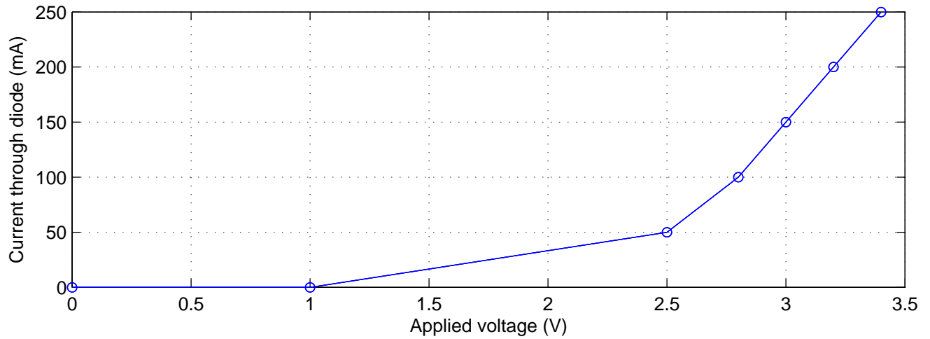
I-V characteristics of Thorlabs DL3147-60 laser diode
