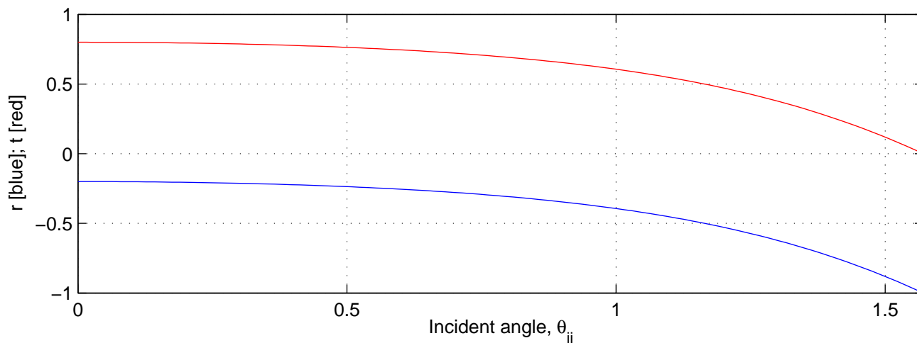
Reflection and transmission coefficients for TE wave
