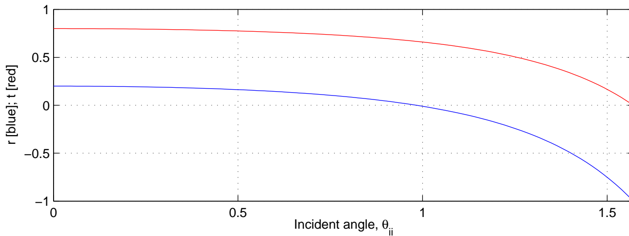
Reflection and transmission coefficients for TM wave
