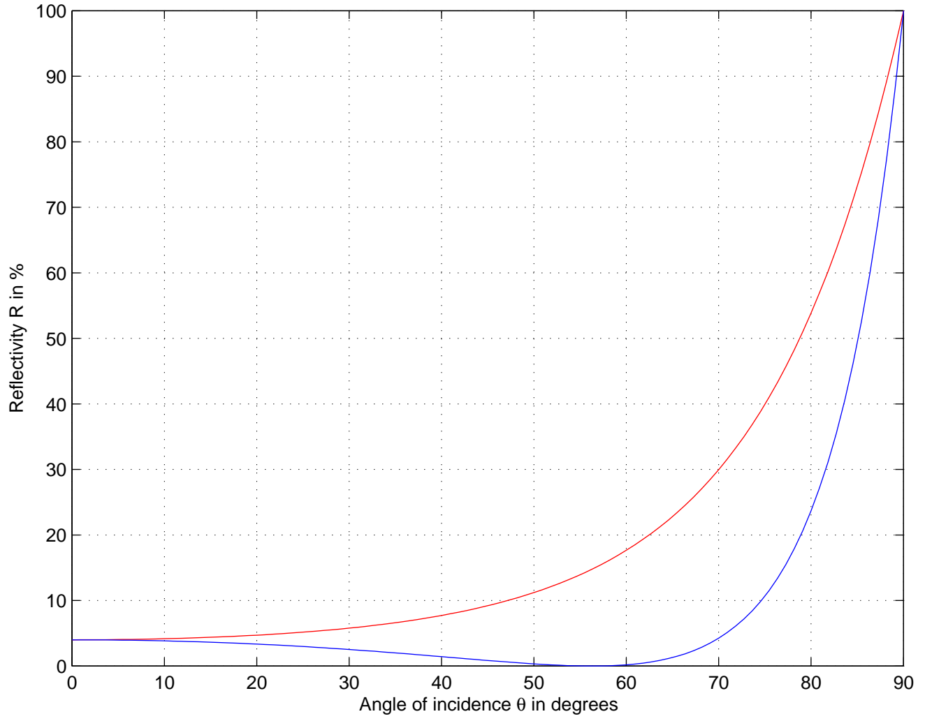
Reflectivity for external reflection on air( n=1 )/glass( n=1.5 ) boundary
