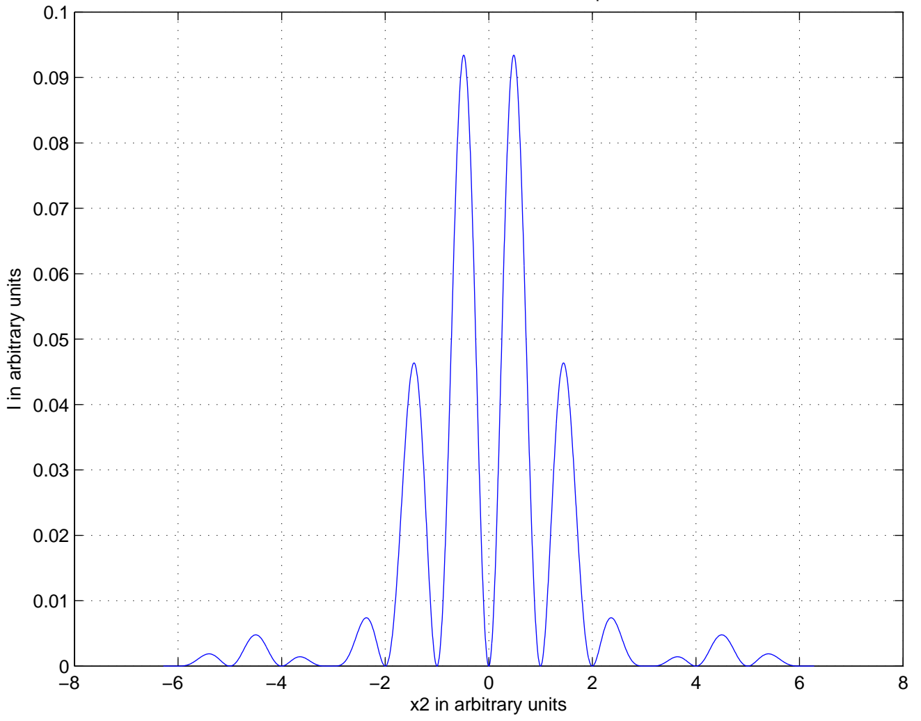
Problem 4.3: Fraunhofer diffraction from a phase-sandwich
