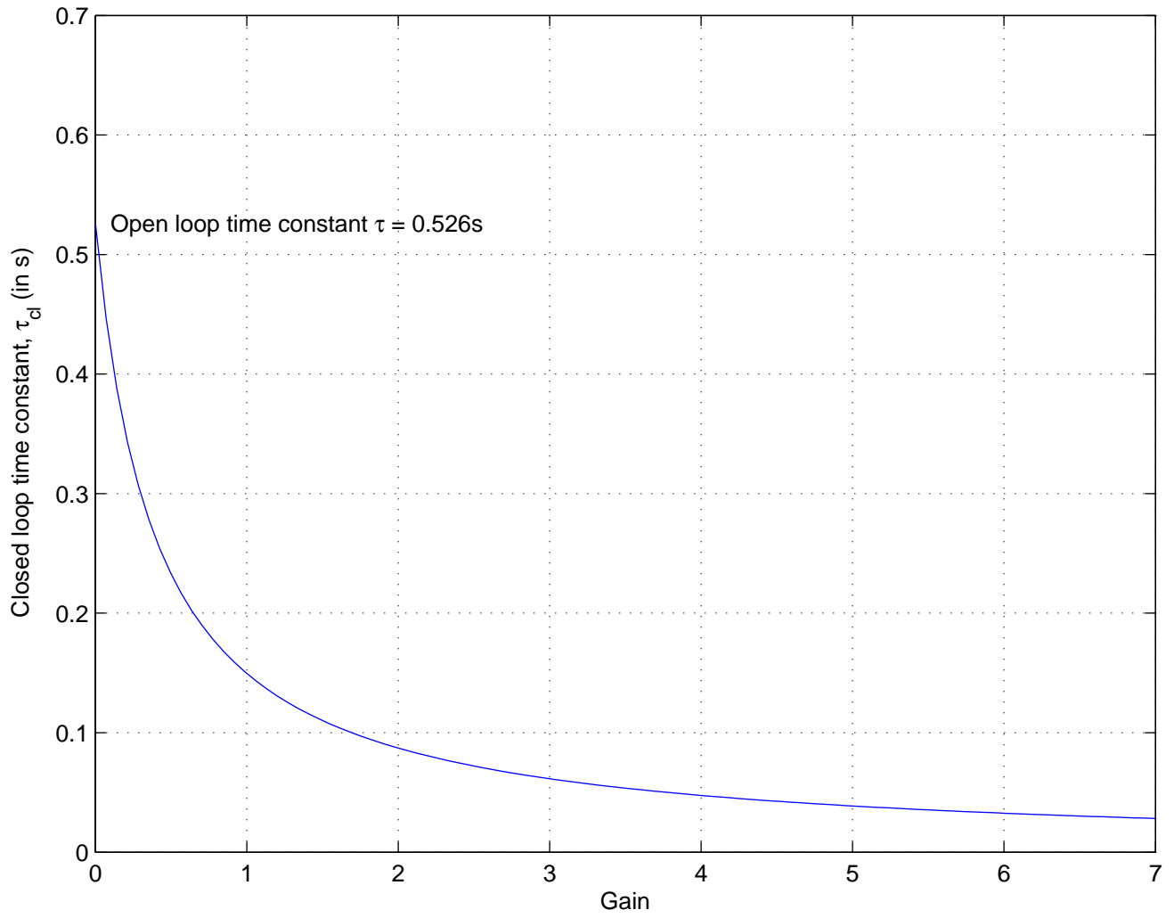
Dependence of \tau_{cl} on compensator gain G
