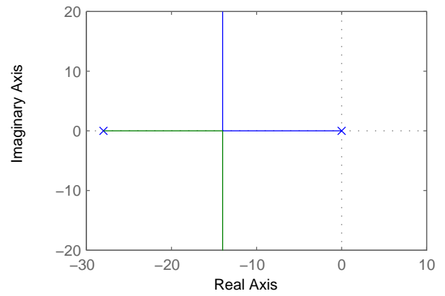
Root locus for G2 = 3.400000\text{e}+000
