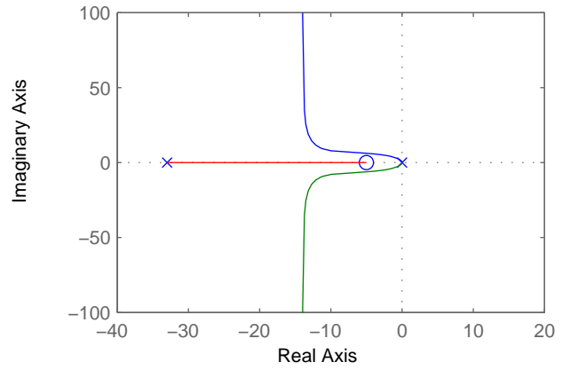
Root locus for G2 = 3.4e+000
