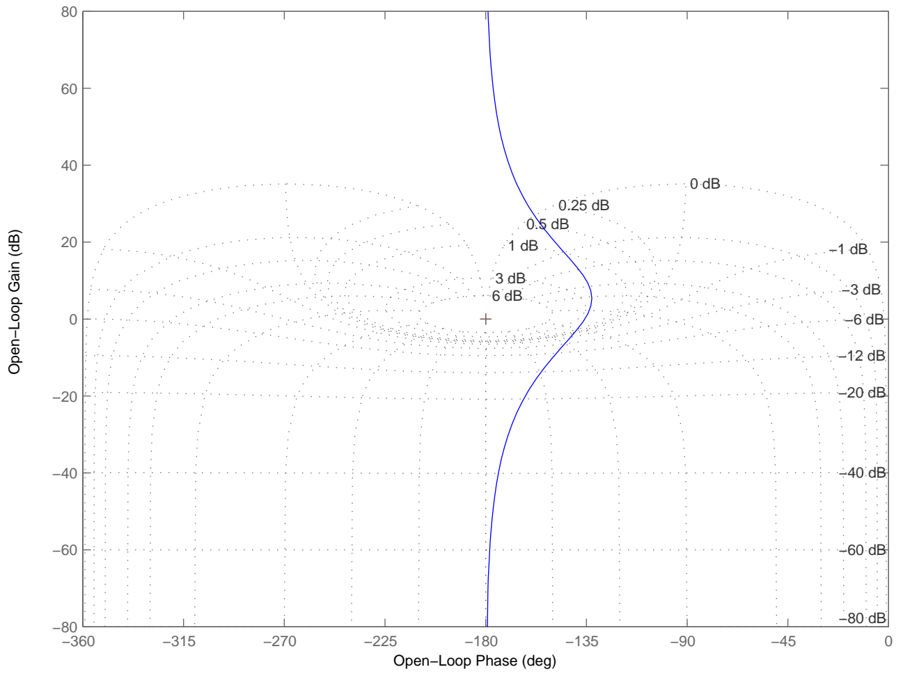
Nichols Chart
