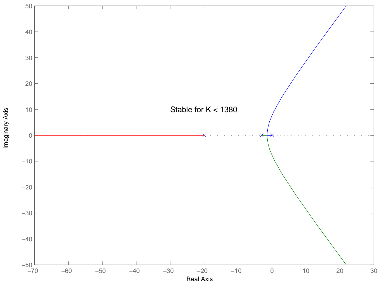
Problem 5a: Root-locus for G_c = H = 1
