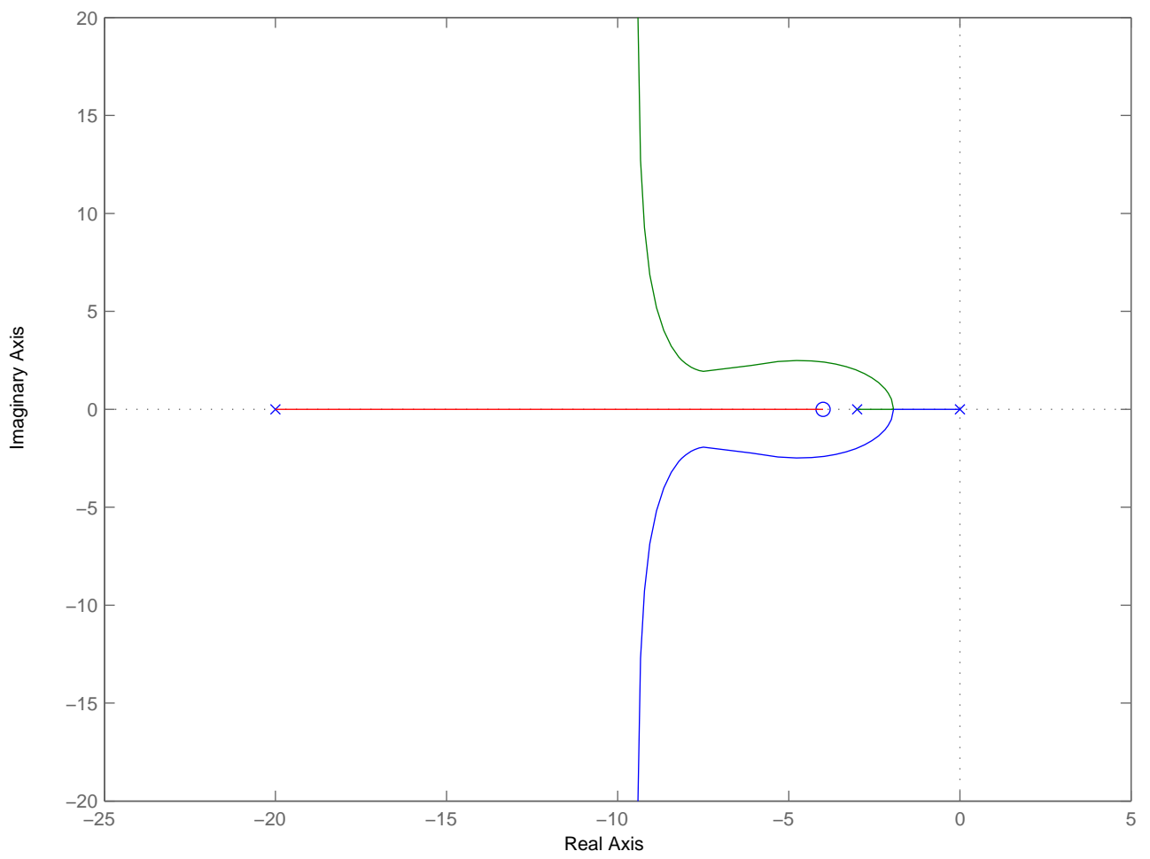
Problem 5bc: Root-locus when G_c * H = (s+4)
