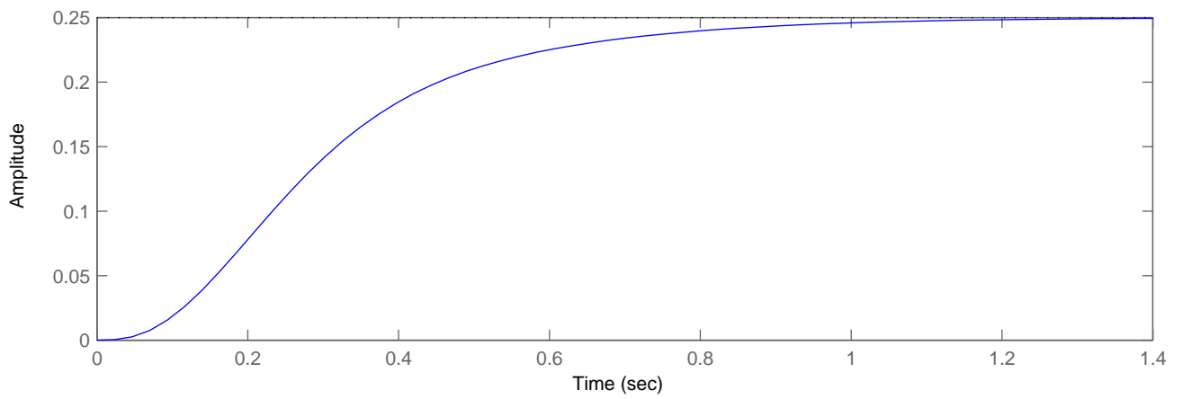
Problem 5c: Step response of G_c=1 , H(s)=s+4
