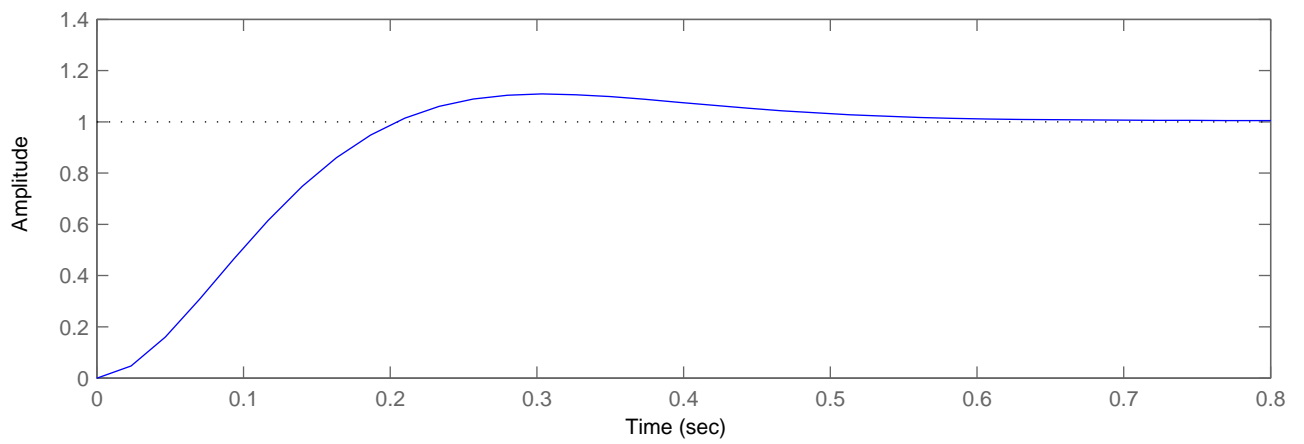
Problem 5b: Step reponse of G_c(s)=s+4 , H=1
