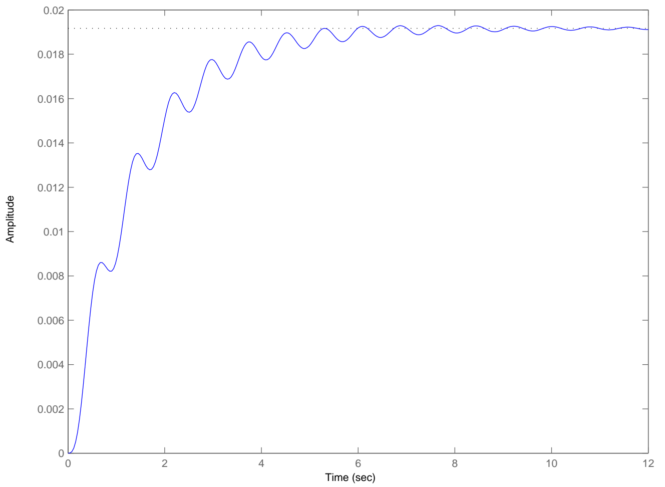
Problem 7c: Step response of C/R, K=1
