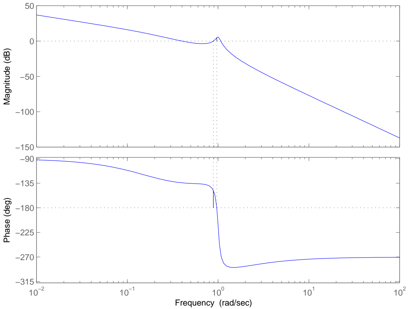
Bode Diagram Gm = -4.81 dB (at 0.968 rad/sec) , Pm = 31.8 deg (at 0.888 rad/sec)
