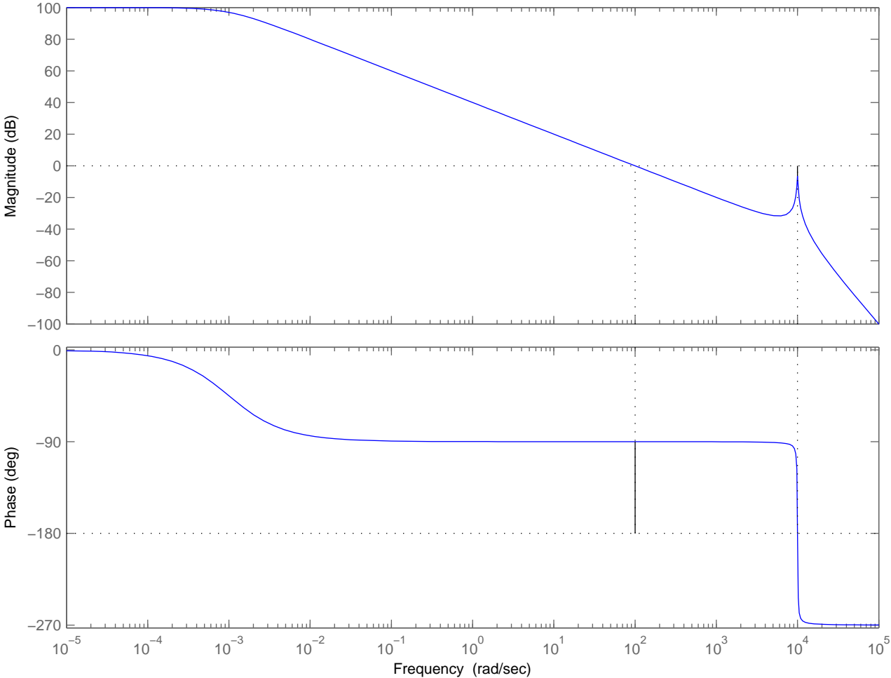
Bode Diagram Gm = 6.45 dB (at 1e+004 rad/sec) , Pm = 90 deg (at 100 rad/sec)
