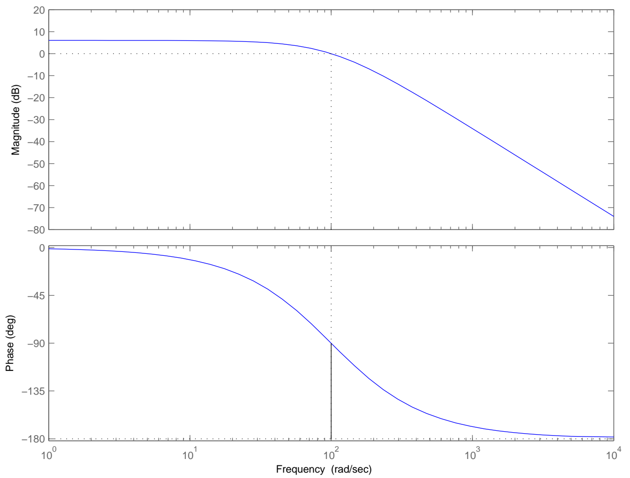
Bode Diagram Gm = Inf dB (at Inf rad/sec) , Pm = 90 deg (at 100 rad/sec)
