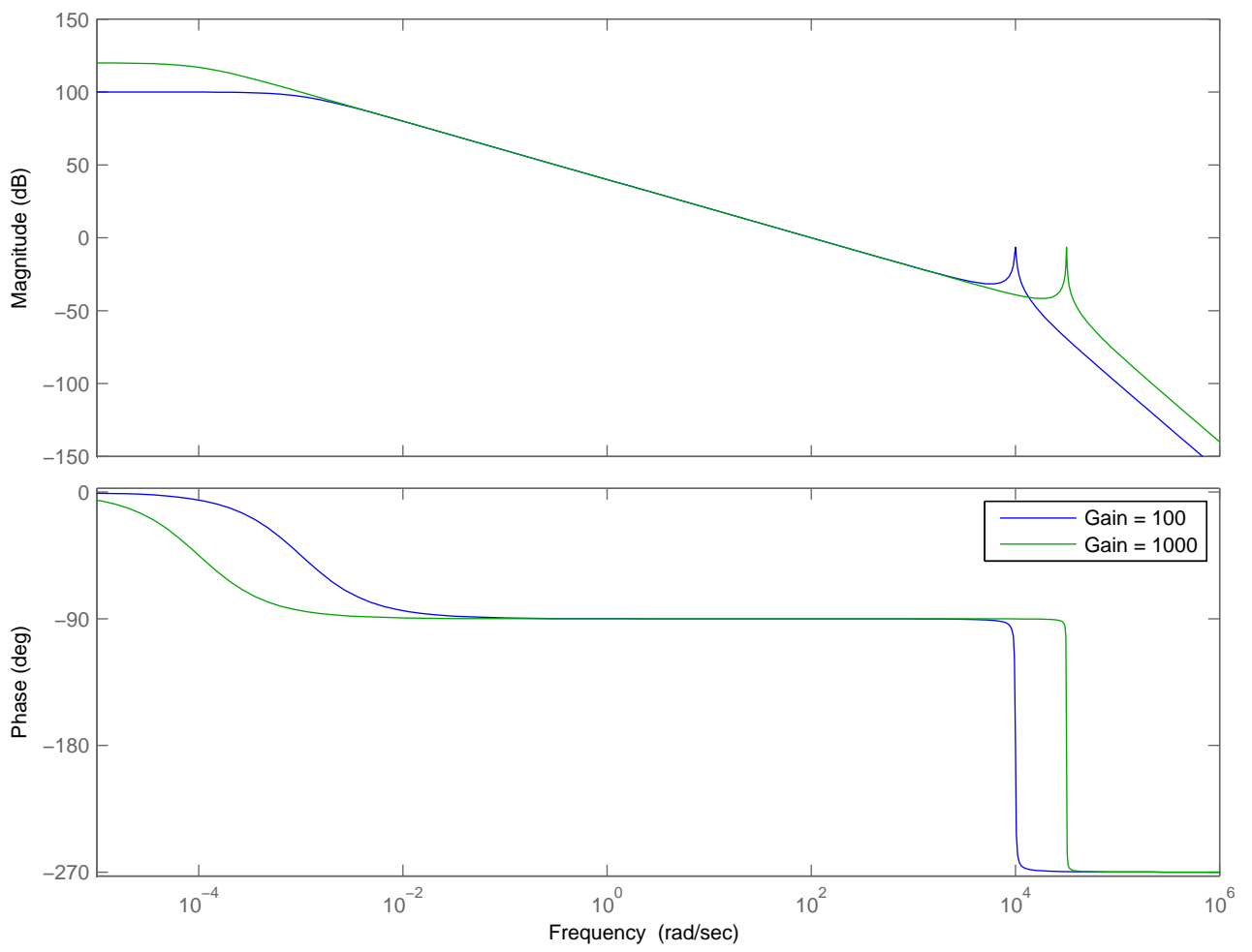
Effect of G_2(s) DC gain (100 vs. 1000) on the minor-loop-compensated loop TF
