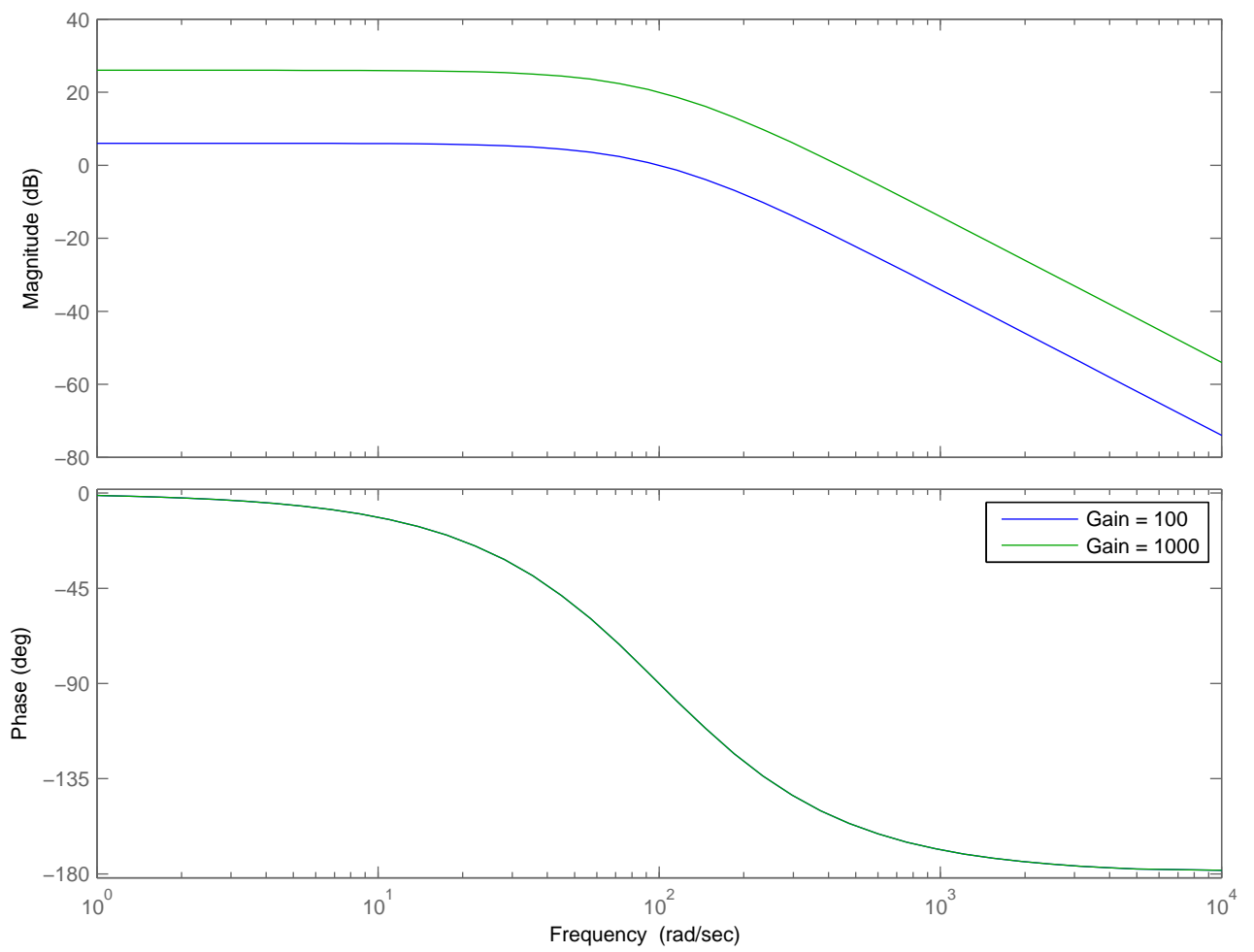
Effect of G_2(s) DC gain (100 vs. 1000) on the series-compensated loop TF
