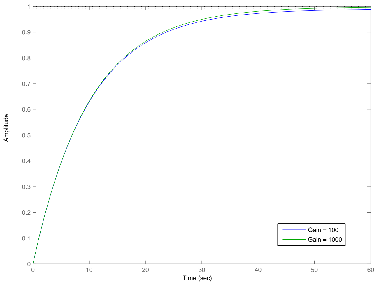
Effect of G_2(s) DC gain (100 vs. 1000) on the minor-loop-compensated step response
