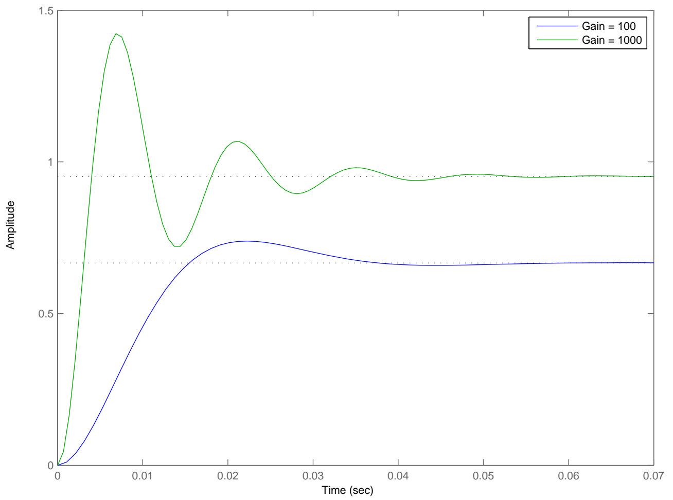
Effect of G_2(s) DC gain (100 vs. 1000) on the series-compensated step response
