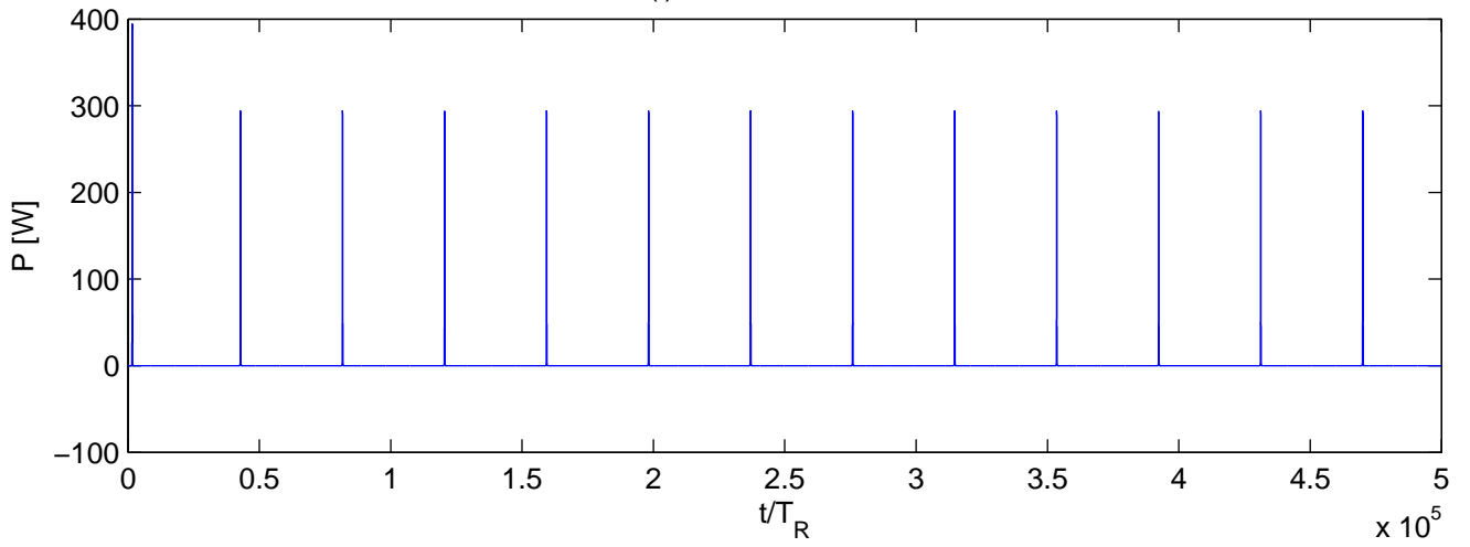
Case (i): Fast saturable absorber
