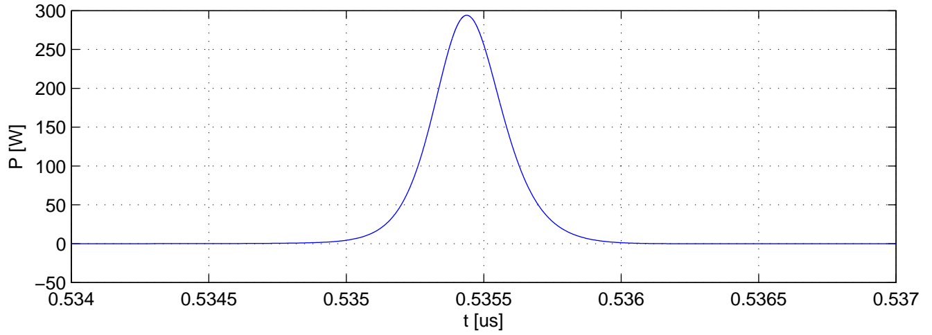
Case (ii): Slow saturable absorber
