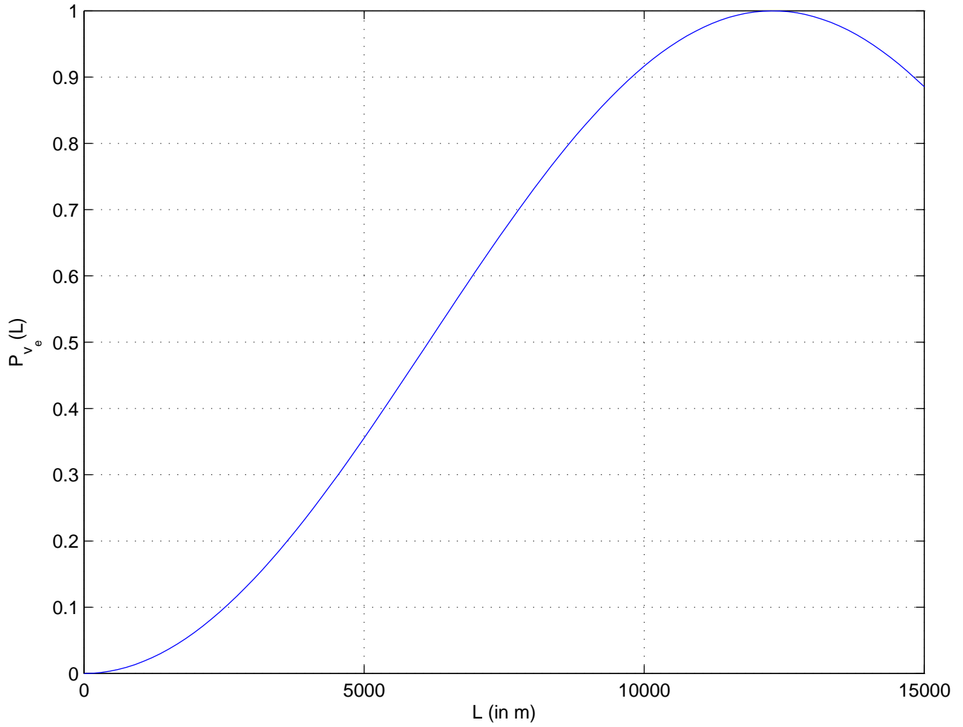
8.05 PS#7 P2(d): Fermilab probability oscillation
