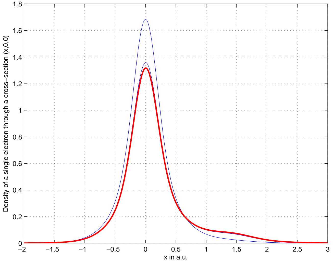
Ground state wavefunction for HeH+. Red indicates the converged solution
