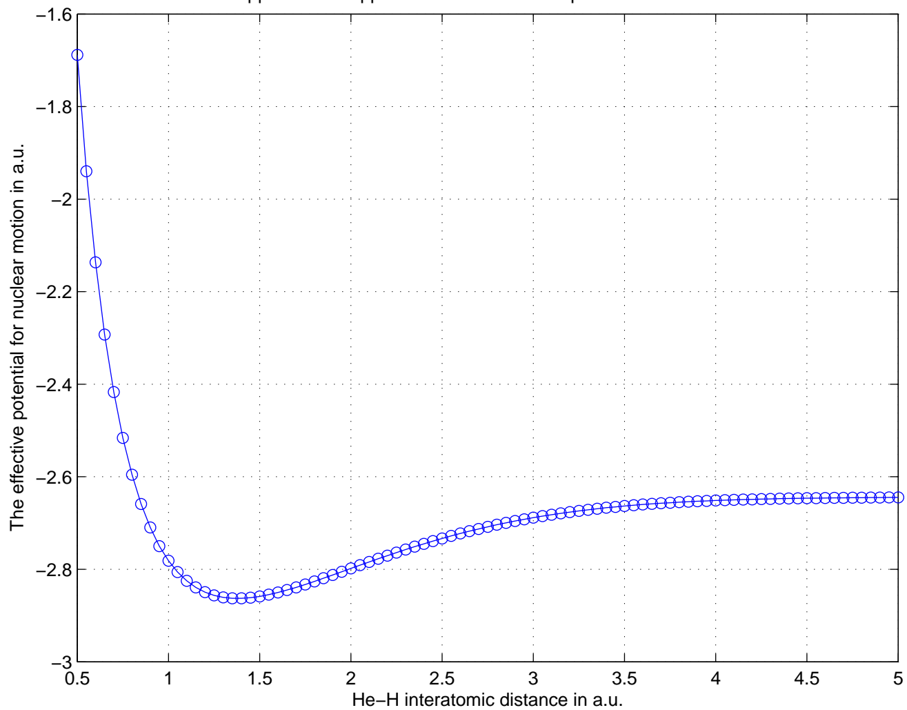
The HF/Born–Oppenheimer approximation for effective potential of nuclear motion of HeH +
