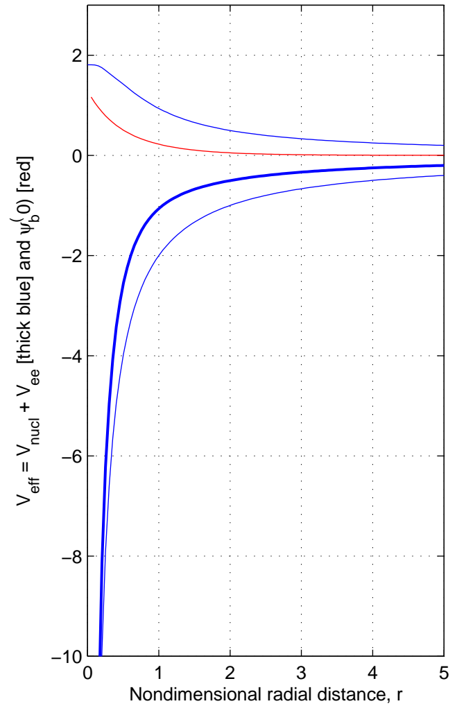
(b) Corresponding wavefunction assignment to electron 2
