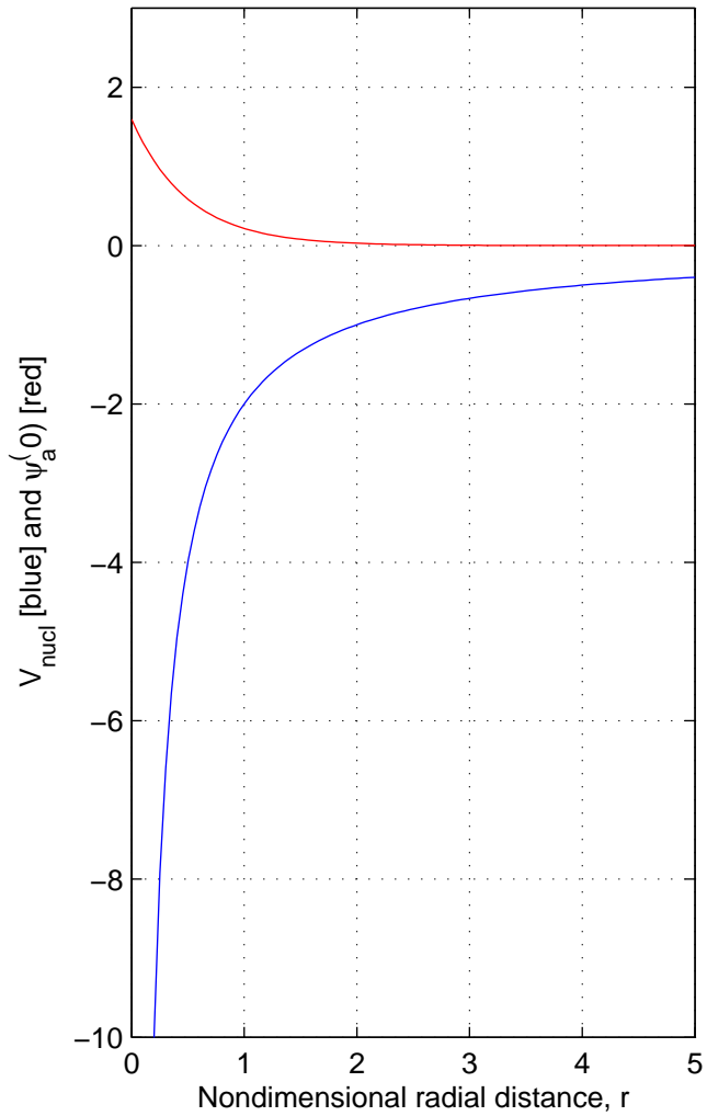
(a) Initial wavefunction assignment to electron 1
