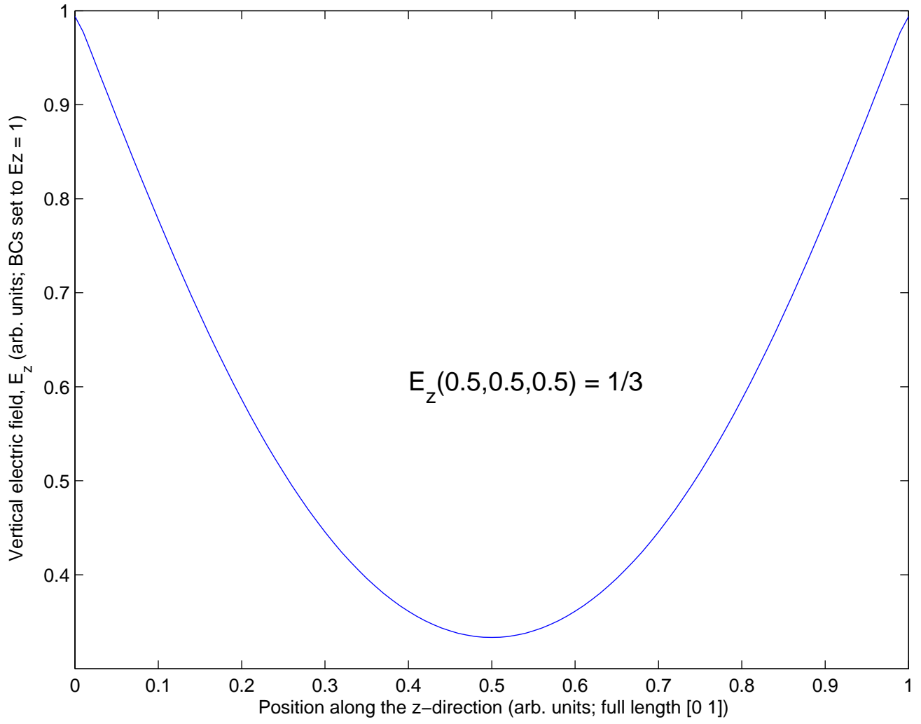
Electric field along the line (x,y,z) = (0.5,0.5,z)
