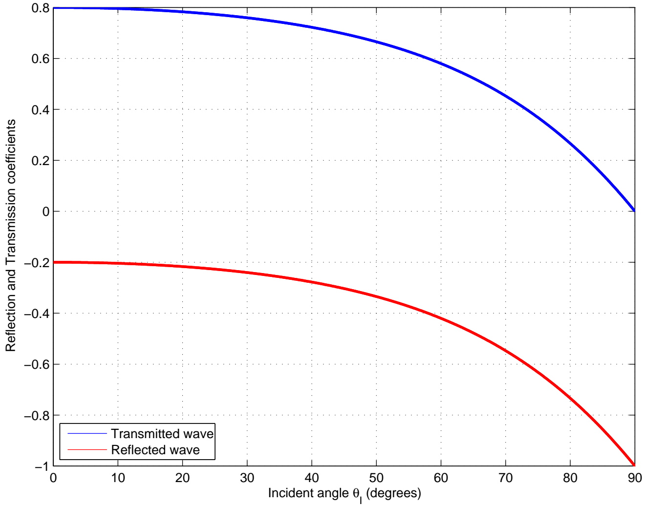
Fresnel equations for TE mode incidence ( n_2/n_1 = 1.5 )
