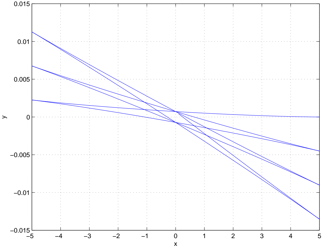
8.09 PS#8, P2: Foucault pendulum in the first minute
