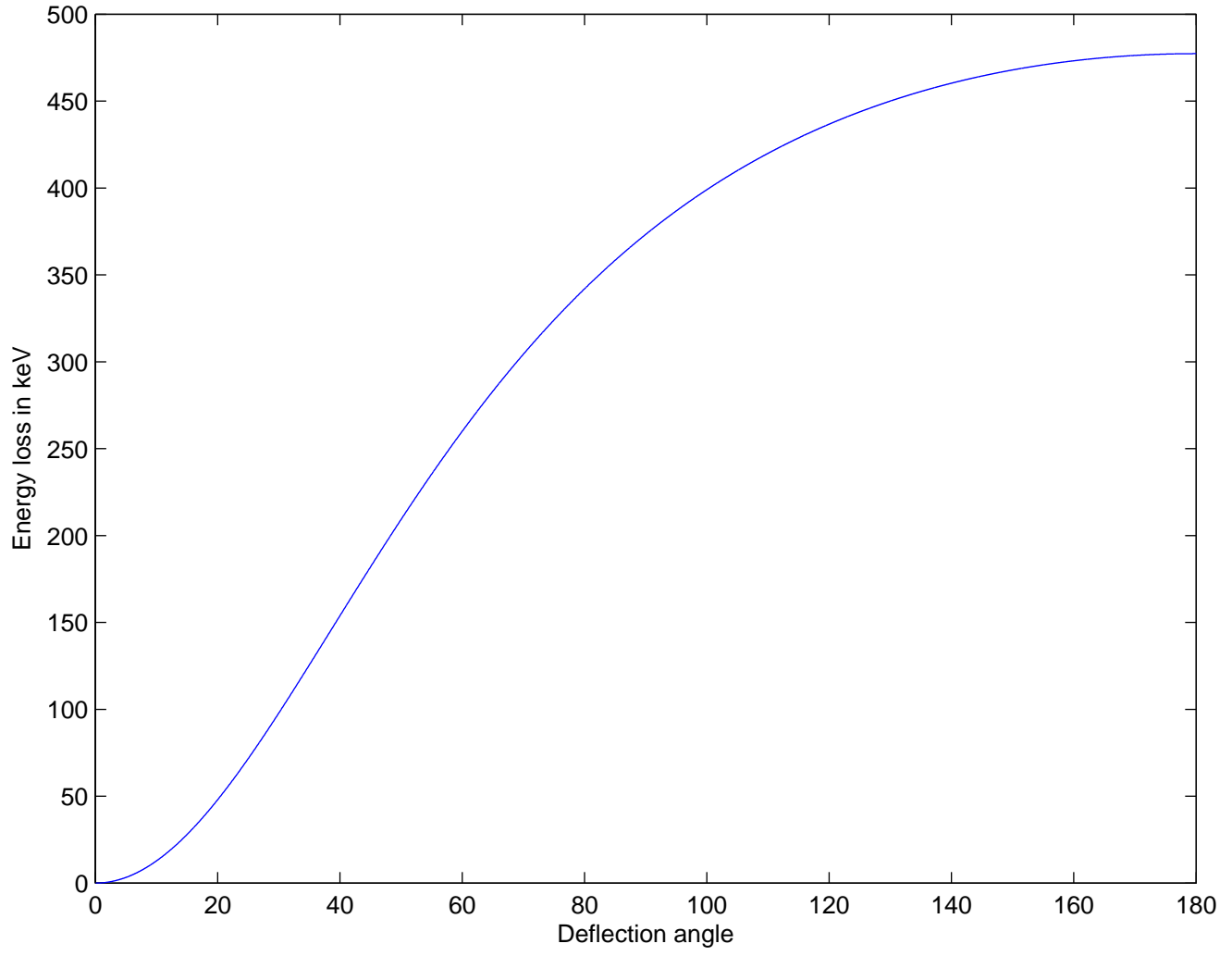
Compton scattering
