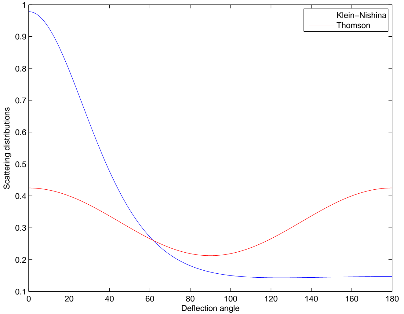
Compton scattering
