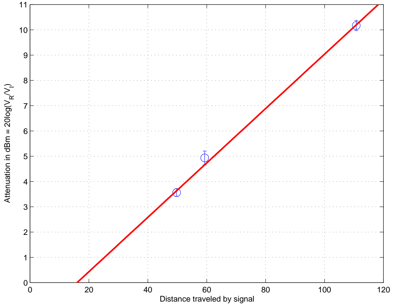
Attenuation of pulse amplitude as function of distance
