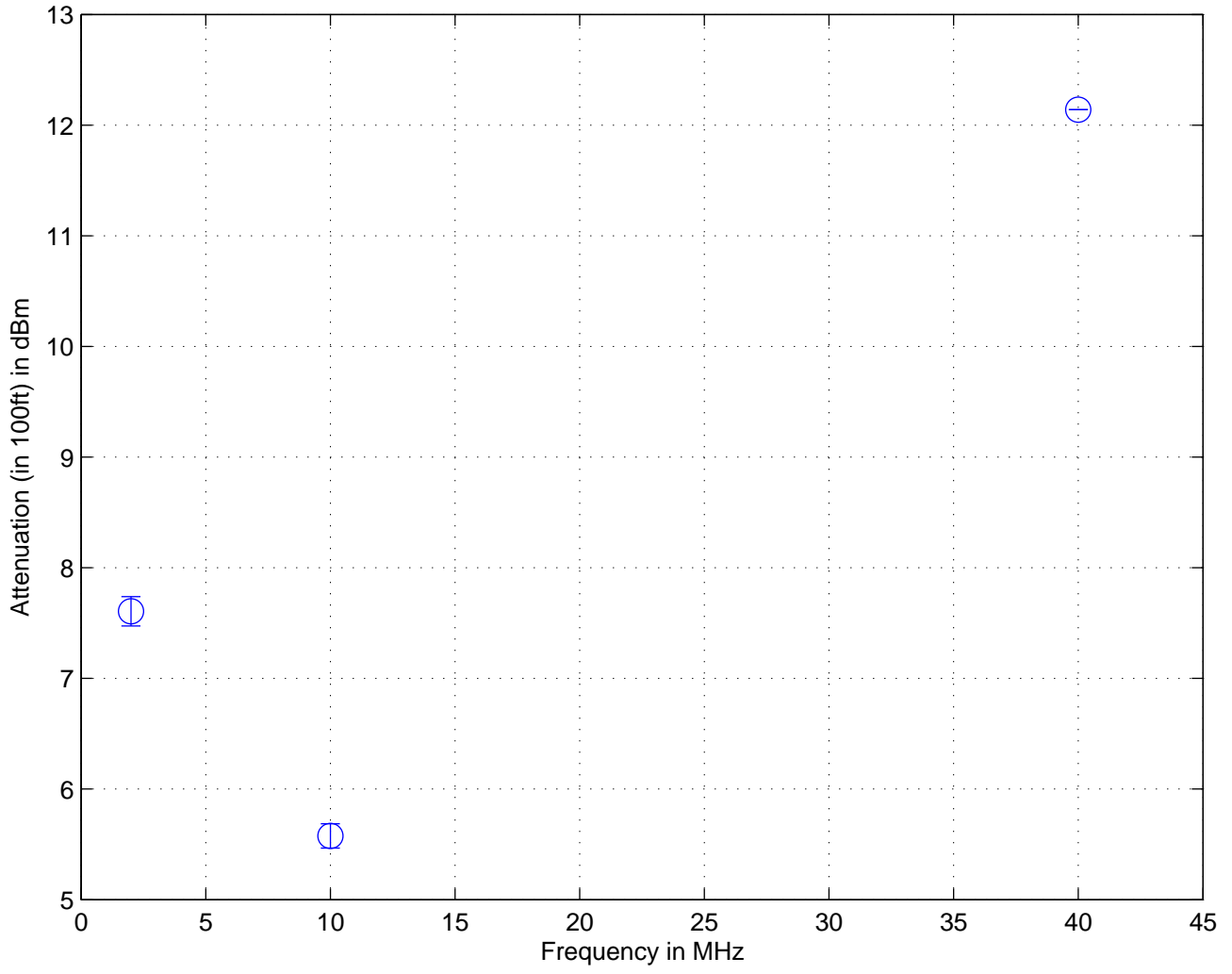
Frequency dependent attenuation in RG58 cable
