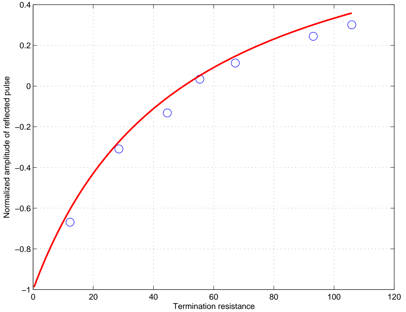
Reflections from cable as a function of termination resistance
