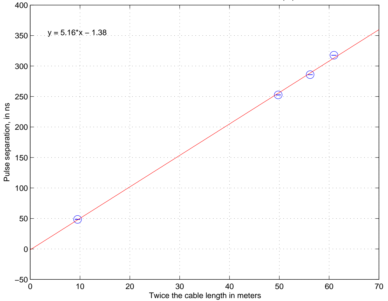
Experiment to determine speed of propagation V_{prop}
