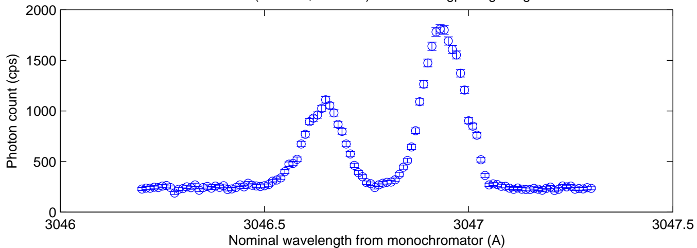
Doublet (3131.55, 3131.84) on the 3600g/mm grating
