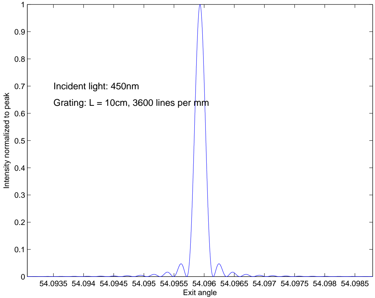
Diffracted light intensity in first order of Littrow configuration
