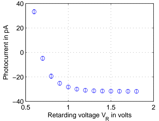
Photocurrent vs retarding voltage for 436nm incident light
