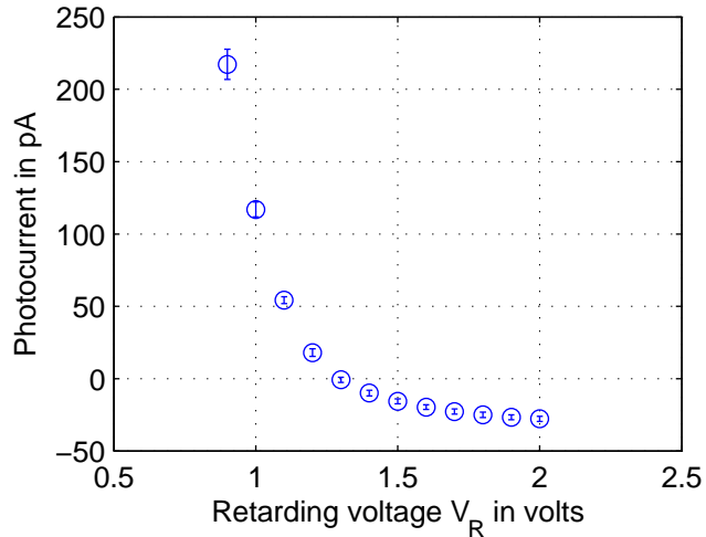
Photocurrent vs retarding voltage for 365nm incident light
