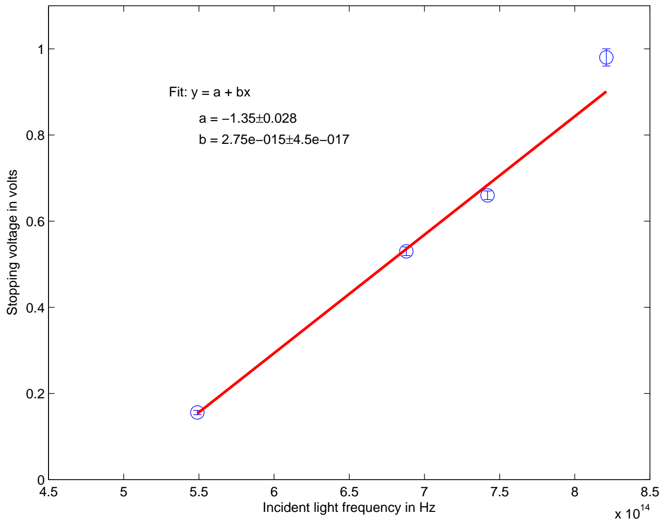
Stopping voltage as a function of incident light freq.
