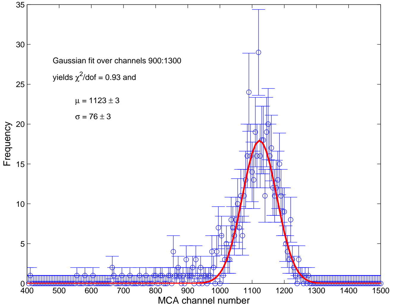
Histogram of \alpha -particle scattering at 10^\circ over 60.50s
