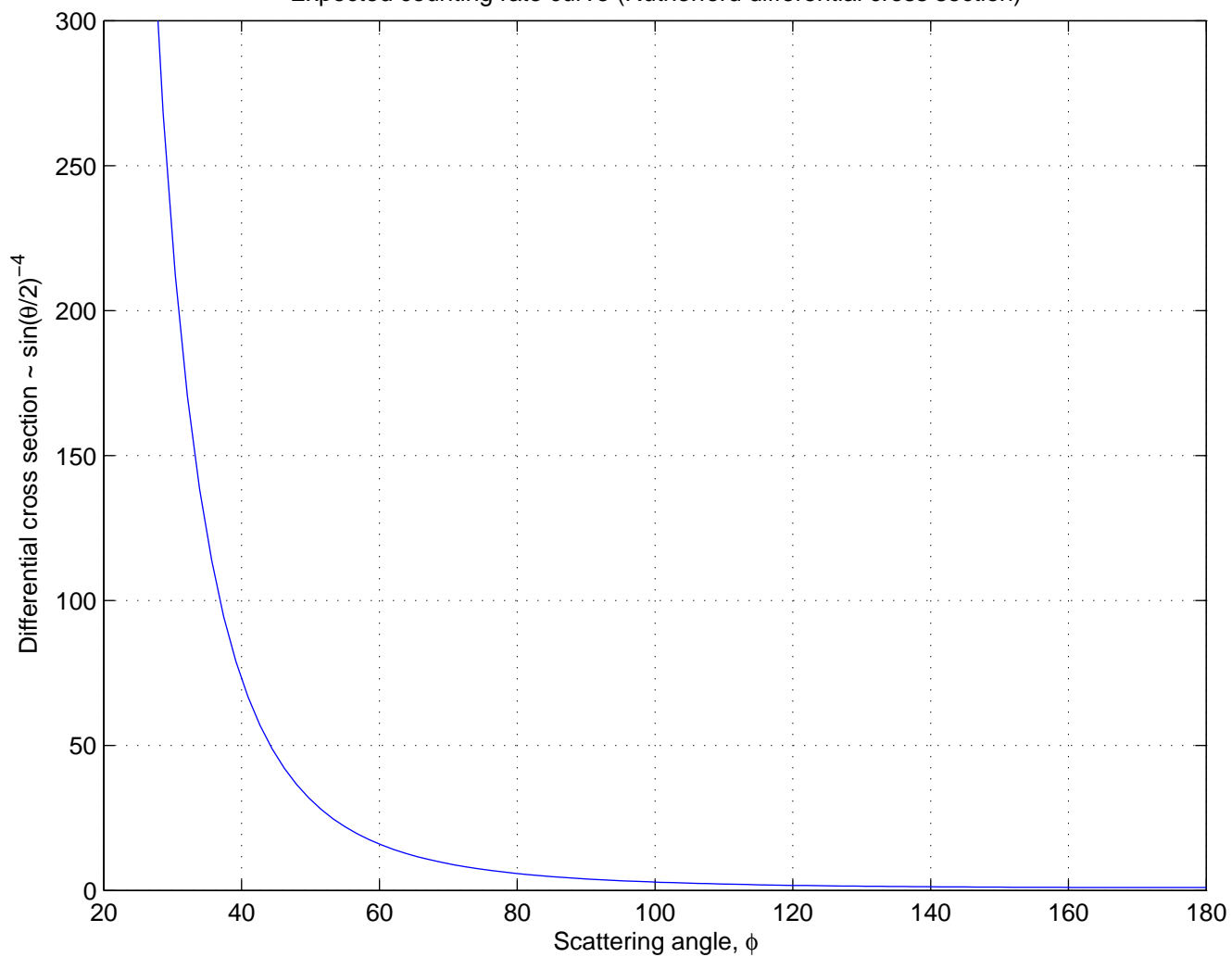
Expected counting rate curve (Rutherford differential cross section)
