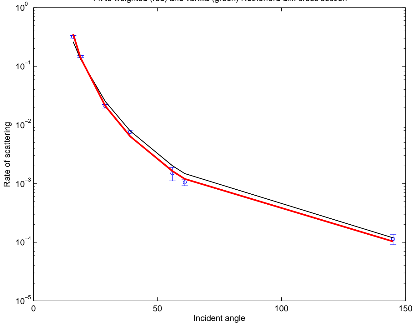
Fit to weighted (red) and vanilla (green) Rutherford diff. cross section
