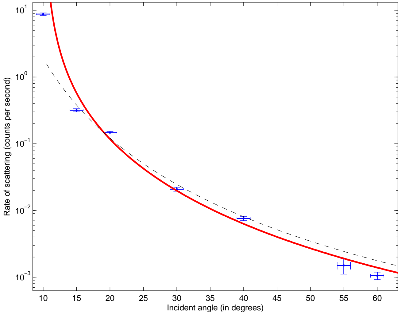
Fits to weighted (red) and vanilla (black) Rutherford diff. cross sections
