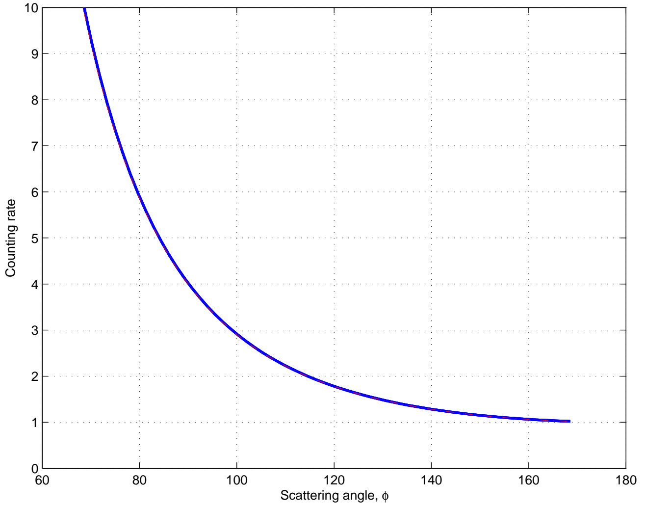
Expected counting rate curve, as given by a triangular angular response function
