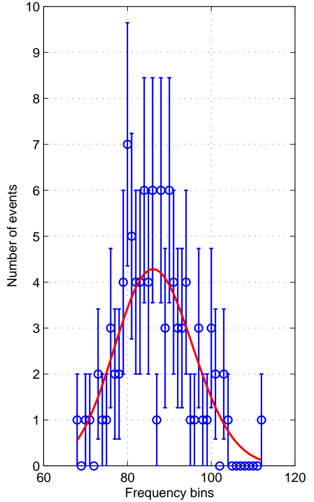
Poisson ~100Hz data and theor. distr.
