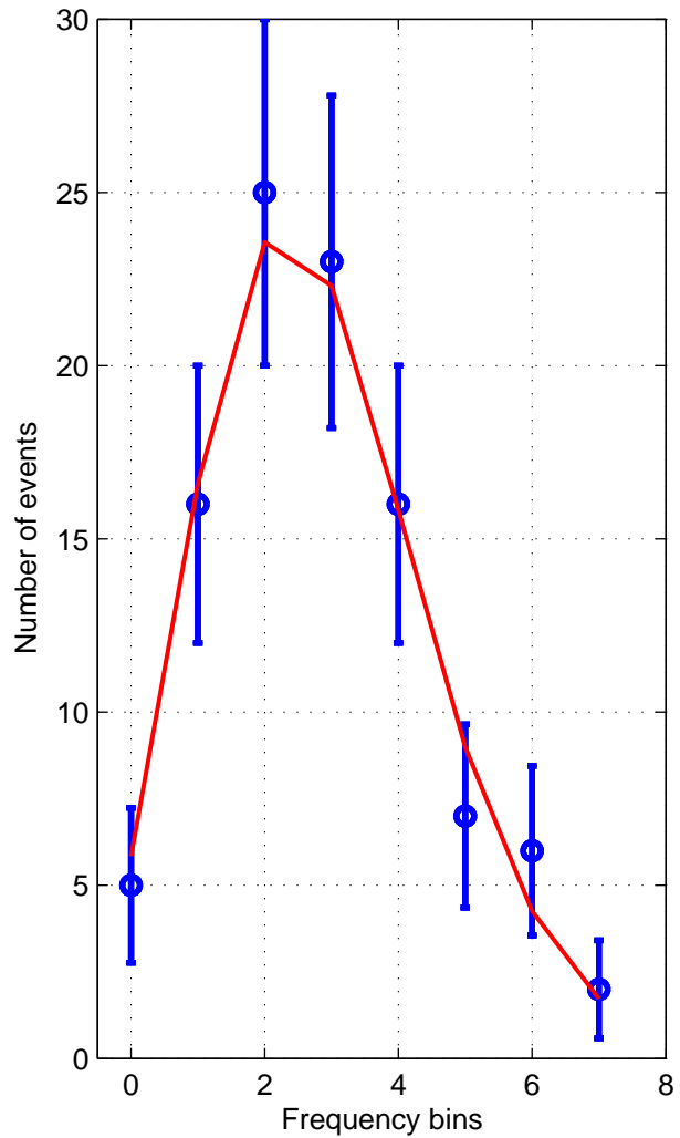
Poisson ~4Hz data and theor. distr.
