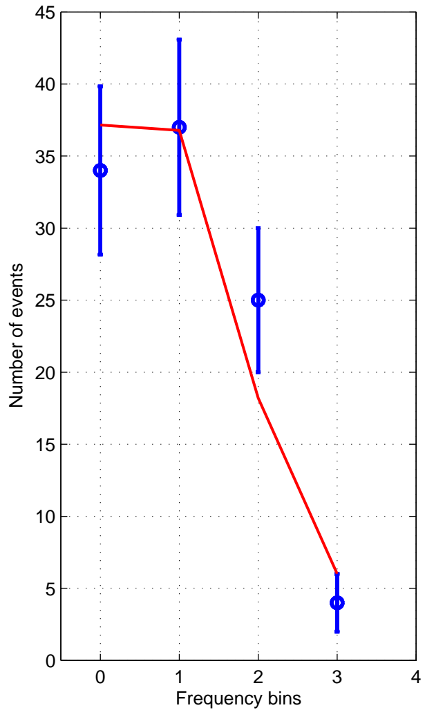
Poisson ~1Hz data and theor. distr.
