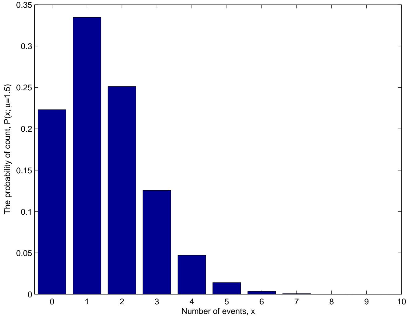
Poisson distribution with \mu = 1.5
