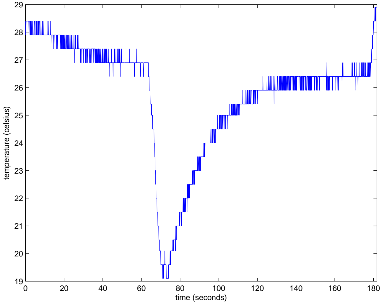
Temperature of LM35; After 1 minute, I sprayed cold air
